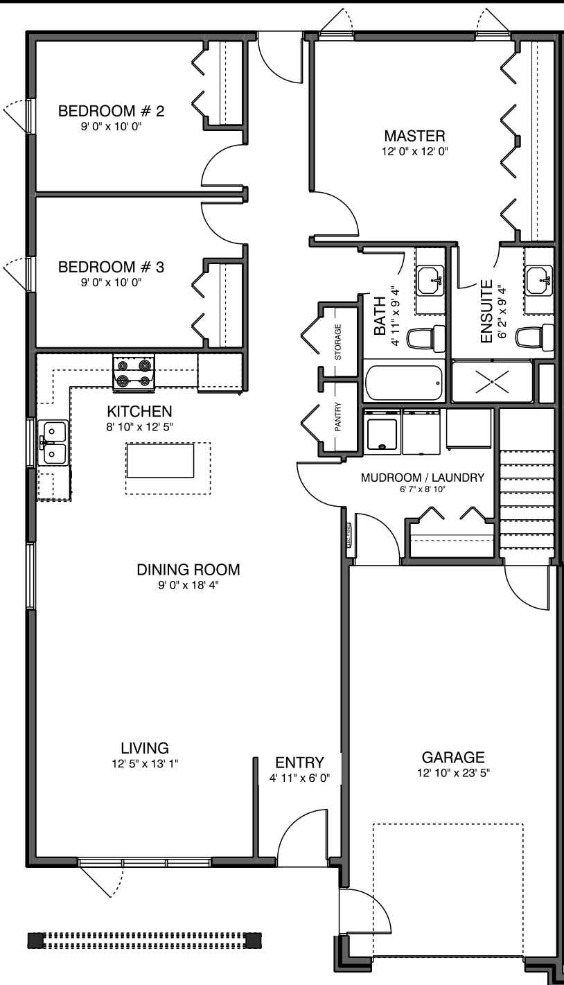
UNIT #109 - MAIN FLOOR
