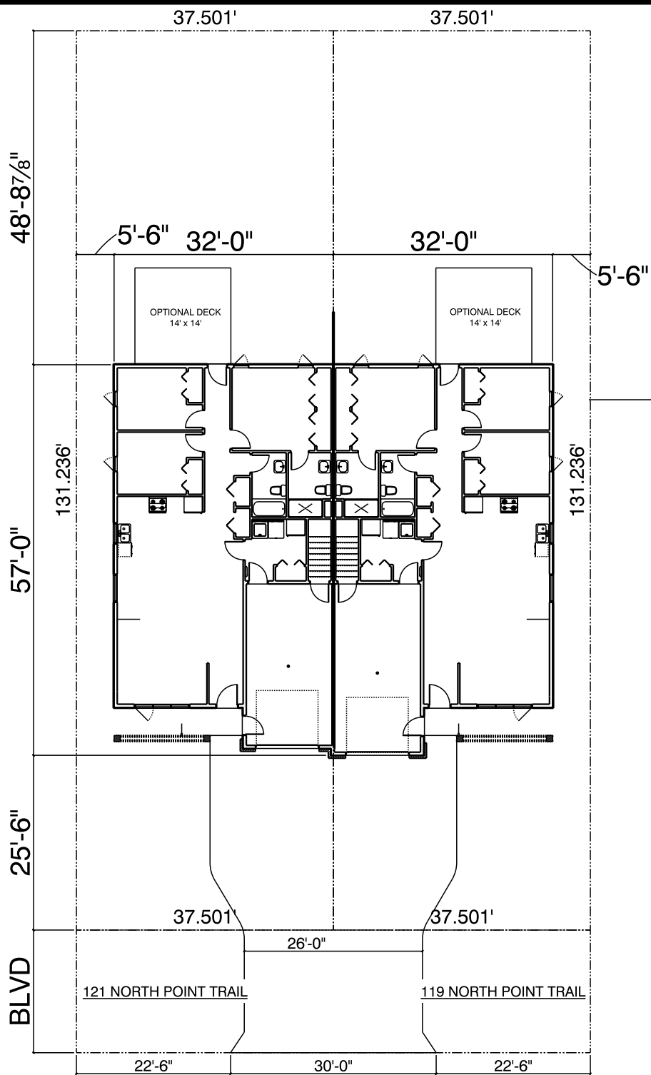
SITE PLAN
